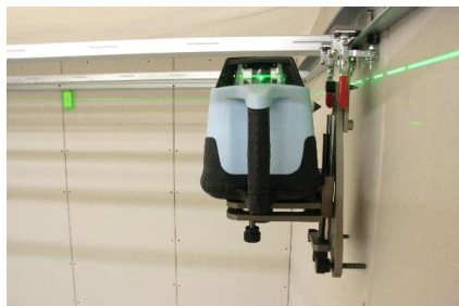
Better visualization of the laser line indoors due to the green laser diode.
