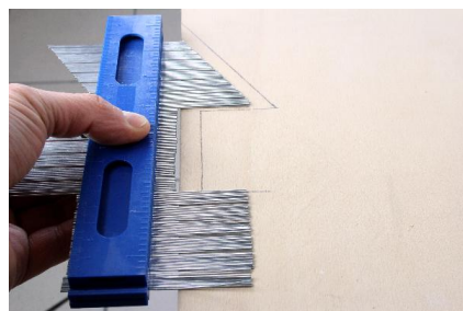
The scanned profile line can be easily transferred to a workpiece thanks to the flat support
