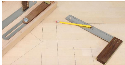
Removal and transfer of angles
