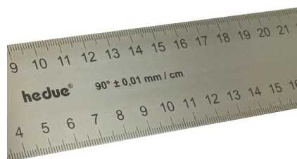
Etched, abrasion-resistant millimetre scale on both sides of the steel tongue
